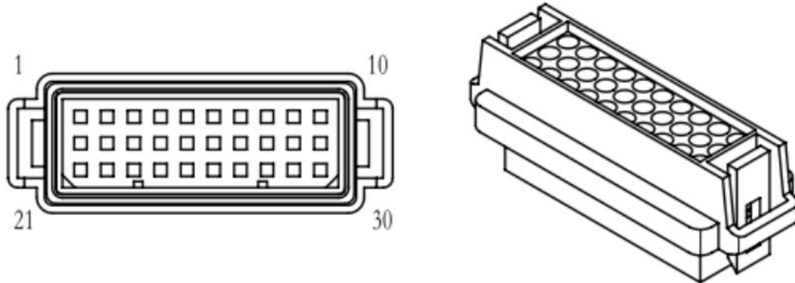
Controller Interface Definitions (30Pin, ZT2023 1.1 × 1.1 × 19.3) (female end ZT2024-A)
